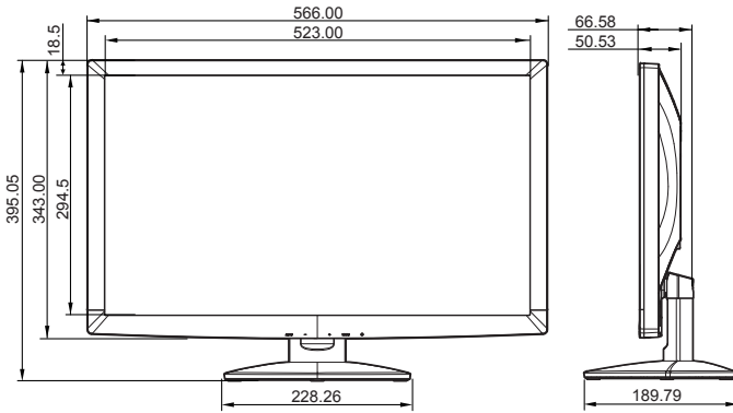
PTFBYF-22W / PTFBNF-22W 寸法図
