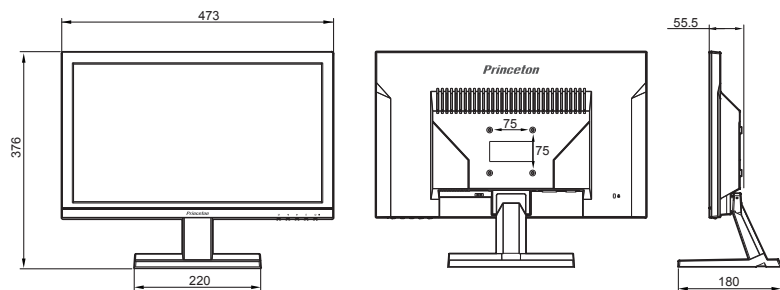
PTFBKF-20W / PTFWKF-20W 寸法図
