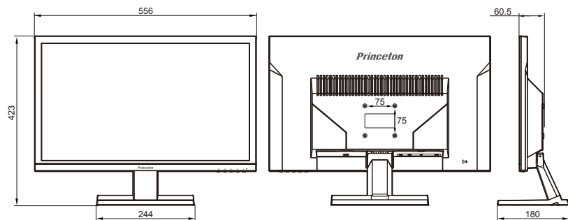
PTFBKF-22W / PTFWKF-22W 寸法図
