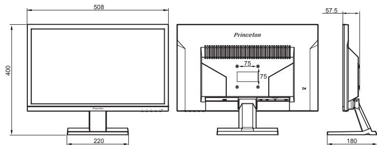
PTFBKF-20W / PTFWKF-20W 寸法図
